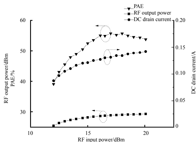
Fig.5 Results of measurement, gate bias voltage is -2.7\text{ V} and drain bias voltage is 10\text{ V} 图 5 栅极偏压为 -2.7\text{ V} ,漏极偏压为 10\text{ V} 时的测量结果
