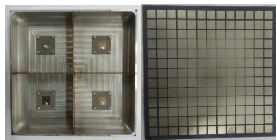
Fig.2 Picture of antenna chamber and reflect plate 图 2 天线腔体与背板结构图
