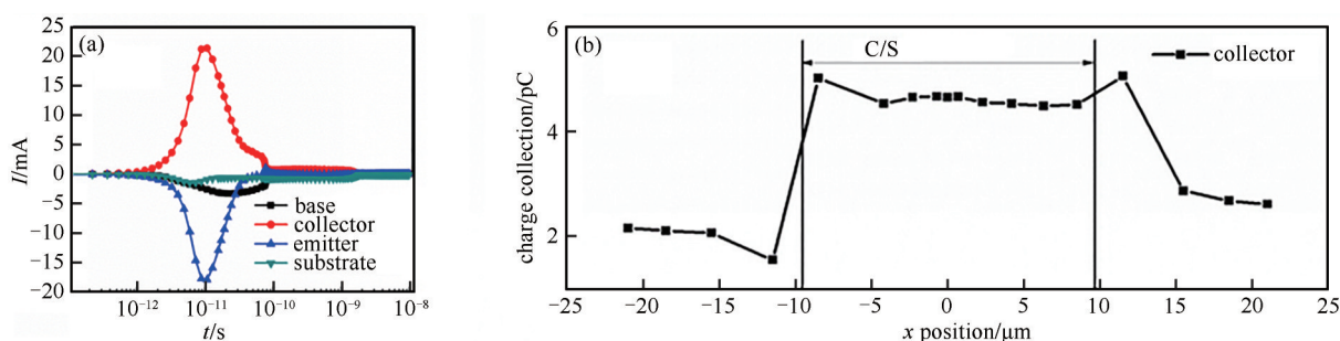
Fig.3 (a) transient currents of different terminals with reverse bias of C/S junction; (b) charge collection of collector in different ion incident positions 图 3 (a) C/S 结反偏条件下各端口电流随时间的变化; (b) 集电极电荷收集量随离子入射位置的变化 [59-60]
