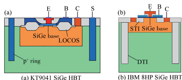
Fig.4 Schematic of device cross section of the SiGe HBTs
