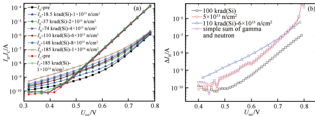
Fig.11 Characteristics before and after irradiation:(a) Gummel characteristics with the total dose and neutron fluence accumulating;
