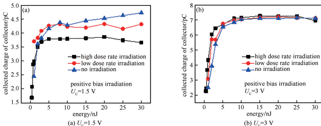
Fig.10 Charge collection versus laser energy after irradiated by high and low dose rates with different biases
