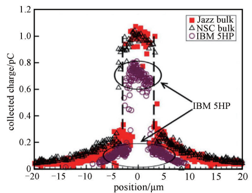
Fig.2 Charge collection of collector in DTI SiGe HBT with different ion incident positions
