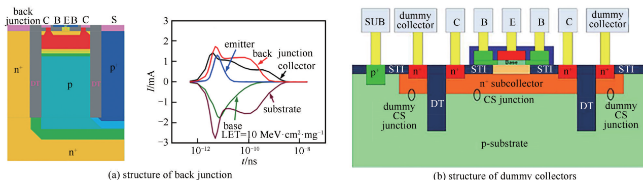
Fig.8 Schematics of radiation hardening
