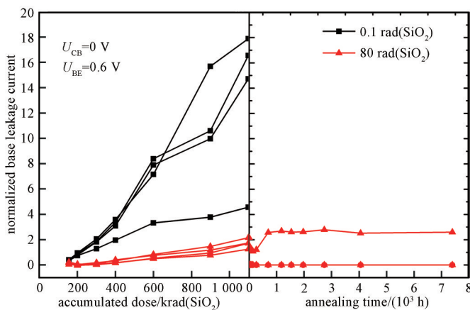
Fig.1 Normalized base leakage current of KT9041 SiGe HBTs for dose rate irradiation and room-temperature annealing as a function of the accumulated total dose
