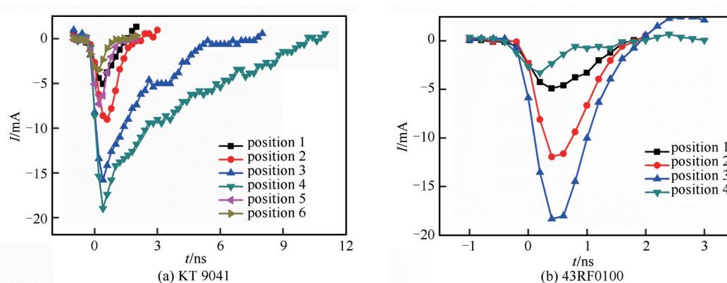
Fig.5 Induced collector transient current with time when laser incoming in SiGe HBTs at different positions
