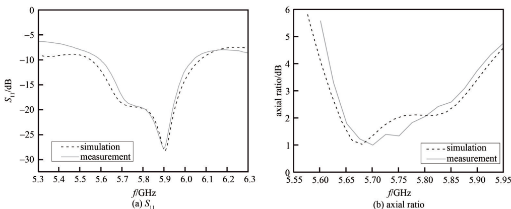
Fig.11 Measured and simulated |S_{11}| and axial ratio of the 1 \times 2 linear array 图 11 1 \times 2 阵列天线 |S_{11}| 及轴比测试与仿真结果
