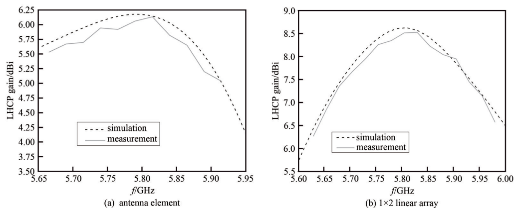
Fig.14 Simulated and measured peak gain of the antenna element and 1 \times 2 linear array
