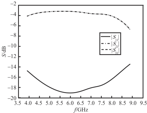
Fig.6 Simulation results of the power splitter 图 6 功分器 S 参数仿真结果
