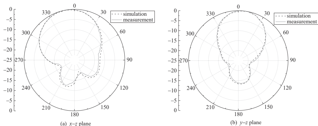
Fig.13 Measured and simulated radiation patterns of the 1 \times 2 array in x - z plane and y - z plane at 5.8 GHz
