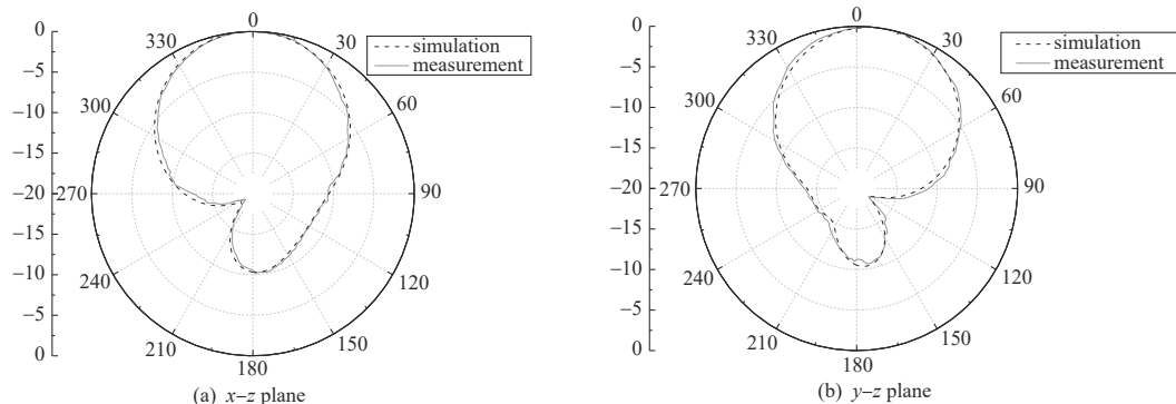
Fig.12 Measured and simulated radiation patterns of the antenna element in x - z plane and y - z plane at 5.8 GHz
